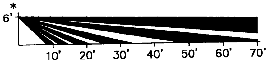
(b) BARRIER LENS, SIDE VIEW.
