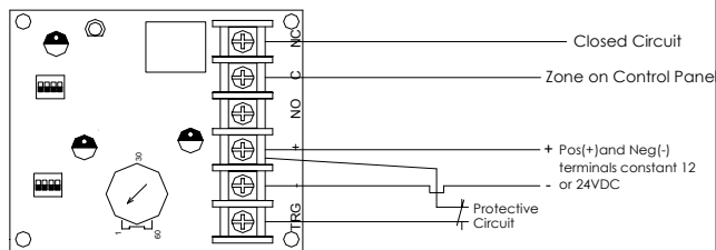
Fig. 3 - Swinger Eliminator:
