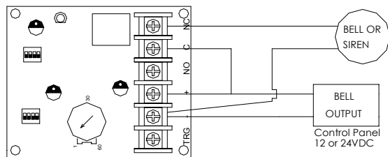
Fig. 7 - Bell Cut Off Timer:
