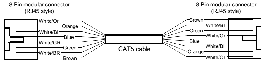
Wiring discipline for Cat 5 connectivity
