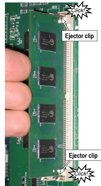
Fig. 4: Seat the module.
